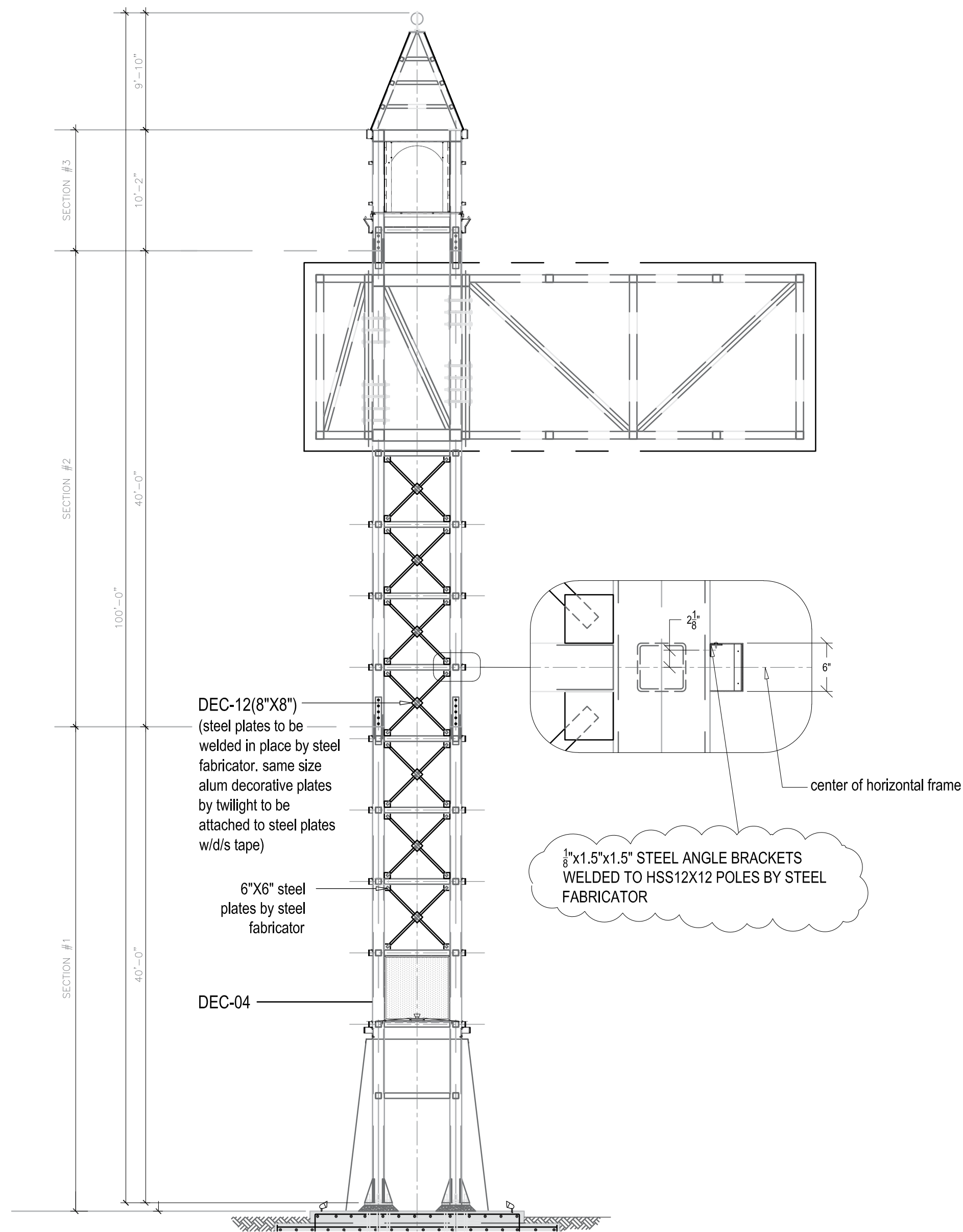
1 A9 DECORATION LAYOUT OF A1 SIGN SCALE: 1:130
